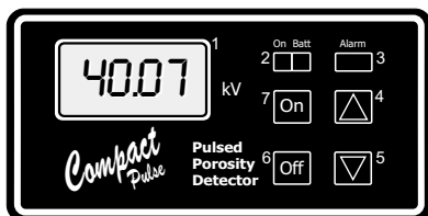
CONTROL LAYOUT
