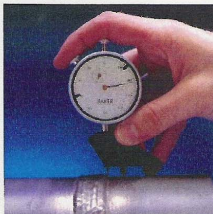
MEASURES UNDERCUT BUTT WELD
