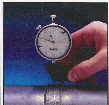
MEASURES CROWN HEIGHT BUTT WELD
