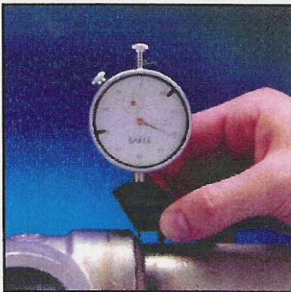
MEASURES UNDERCUT SOCKET WELD
